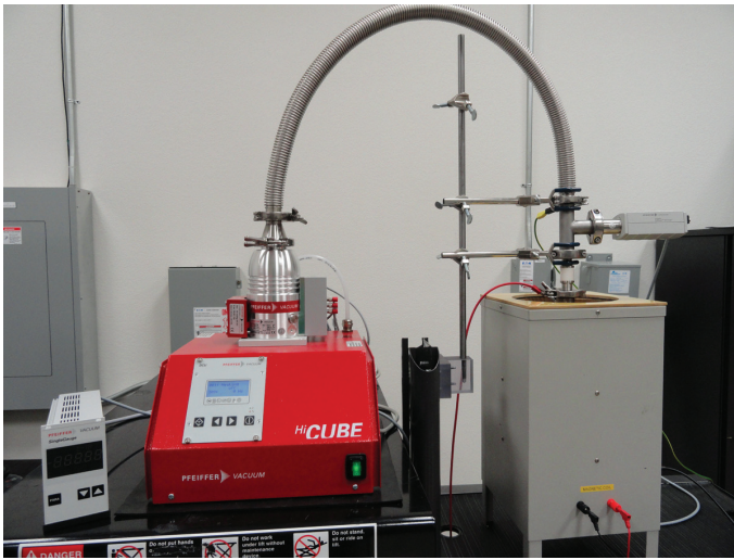
Figure 10. Test setup for developing vacuum versus current data.
